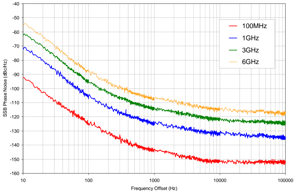
Figure 1: SSB Phase Noise at 100MHz, 1GHz, 3GHz & 6GHz ( P_{OUT}=+12dBm )
